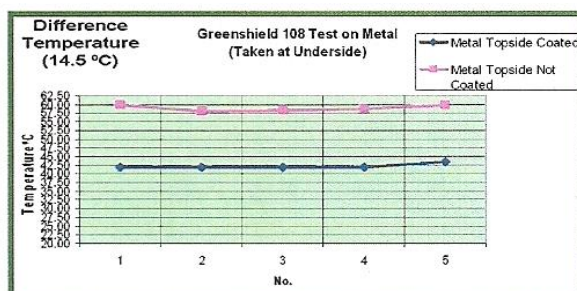
Metal Temperature Analysis (Graph)
