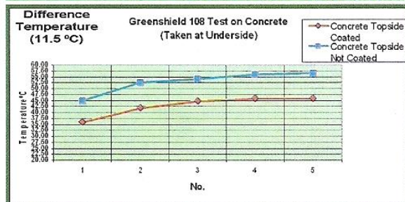
Concrete Temperature Analysis (Graph)
